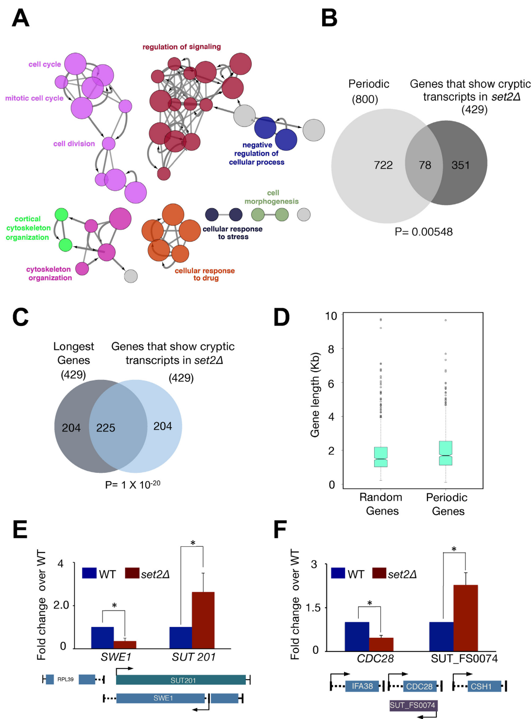
Figure 1. Long genes prone to cryptic transcripts are associated with cell cycle related functions. (A) Network analysis, following pathway enrichment analysis, of genes that give rise to cryptic transcript from (32) showing the ontology relationships between the pathways. Genes that give rise to cryptic transcripts (429 genes from Lickwar et al. (32)) in set2Δ cells reveal an enrichment of these genes with the cell cycle, mitosis, DNA replication and cell polarity. The direction of the arrows shows the ontology of related functional categories. (B) A Venn diagram comparing genes that are periodic (top 800 from Cyclebase) to those that give rise to cryptic transcripts in set2Δ cells reveal a significant overlap ( p = 0.00548 ). (C) Venn diagram showing that genes which give rise to cryptic transcription in set2Δ cells also tend to be long ( P < 1 \times 10^{-20} ). (D) Plot showing the relationship between long genes (800 random genes) and periodic genes (top 800 from Cyclebase) reveal periodic genes tend to be longer than expected by chance ( P < 2.531 \times 10^{-5} Kolmogorov–Smirnov test). (E) and (F) RT-qPCR analysis of sense and antisense transcripts originating from the SWE1 ( SUT201 ) and CDC28 genes ( SUT_FS0074 ), demonstrating the reduced sense transcript levels of SWE1 and CDC28 in set2Δ cells.
