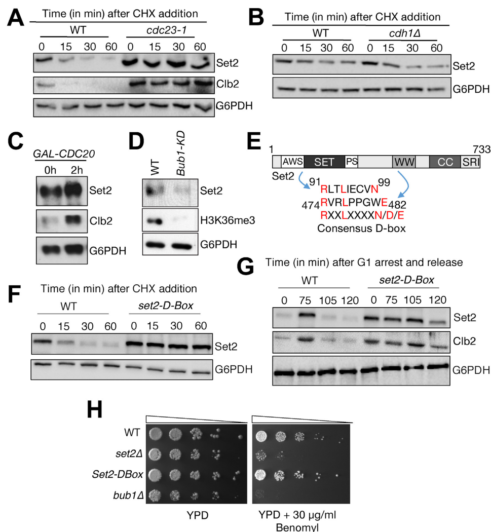
Figure 6. The Anaphase Promoting Complex (APC) promotes Set2 protein turnover across the cell cycle. (A) Compromised APC/C function stabilizes Set2 protein levels. Cycloheximide chase experiments were performed using a WT or APC mutant allele ( cdc23-1 ) after shift to restrictive temperature (37°C), and cell extracts were immunoblotted for Set2. G6PDH was used as a loading control. (B) Set2 is not regulated by APC/C Cdh1 . Cycloheximide chase experiments were performed as described in panel (A) in WT and CHD1 deleted cells ( cdh1Δ ) to detect the rate of Set2 loss. (C) Set2 is regulated by the APC/C Cdc20 . A GAL-CDC20 strain was grown in dextrose for 2 h to shut off expression of CDC20 , and protein extracts were immunoblotted to probe for Set2, Clb2 and G6PDH. (D) An immunoblot showing the decrease in the levels of Set2 and H3K36me3 in a strain that contains a kinase-dead allele of BUB1 , a checkpoint kinase that negatively regulates CDC20 . (E) Representation of Set2 protein showing the domains and two putative D-boxes in the protein sequence. For comparison, a canonical D-box sequence is shown. (F) Mutation of the conserved D-box residues in Set2 (RXXL → AXXA) enhances Set2 stability. Cycloheximide chase experiments were performed at the indicated time points on WT and the D-box mutant strains and probed for Set2 and G6PDH. (G) Set2 protein levels become uncoupled from cell cycle regulation upon D-box mutation. Lysates were prepared from WT and D-Box mutants of Set2 post G1 arrest and released at indicated time points. Lysates were probed for Set2, Clb2 and G6PDH. (H) Appropriate turnover of Set2 protein is required for proper response to mitotic poison, benomyl. Five-fold serial dilutions of indicated strains were spotted on either SC-Ura or SC-Ura with benomyl (30 µg/mL).
