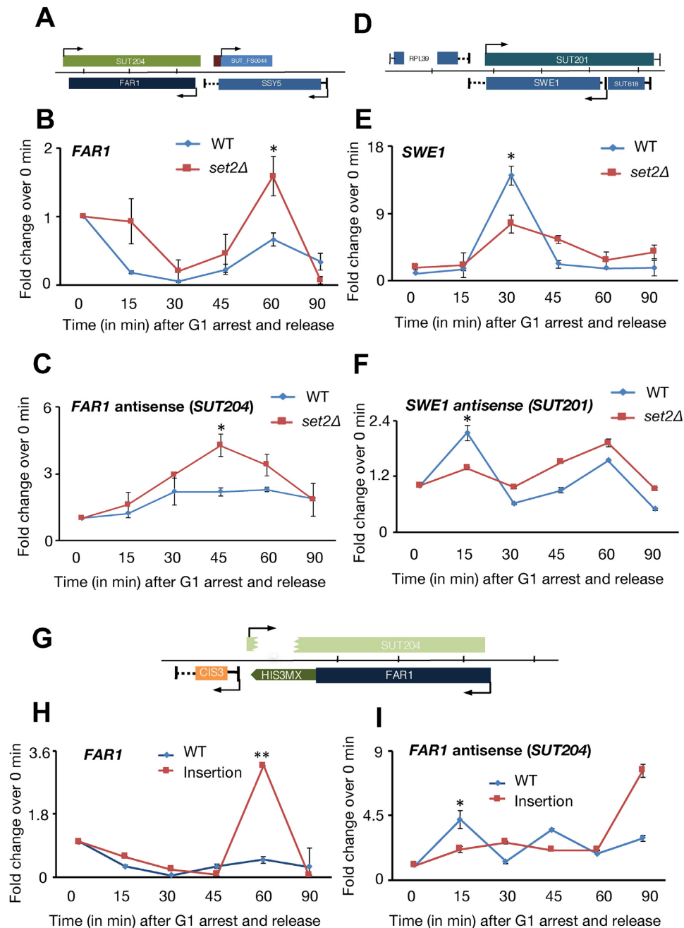
Figure 2. The transcriptional fidelity of cell cycle-regulated genes is maintained by Set2. (A) Diagrammatic representation of the FAR1 locus and its corresponding antisense stable un-annotated transcript ( SUT204 ). (B) qRT-PCR showing the absence of SET2 results in mis-regulation of the levels of both sense and antisense FAR1 transcripts. (C) FAR1 antisense transcript, SUT204 , is increased in set2Δ cells at all points across the cell cycle, as assessed by qRT-PCR. (D) Schematic representation of the genomic locus of SWE1 and its corresponding antisense transcript, SUT201 . (E) Loss of SET2 results in the mis-regulation in the levels of SWE1 sense transcript (compare the levels of SWE1 transcript at 30 and 45 min between WT and set2Δ ). (F) qRT-PCR of SWE1 antisense transcript SUT201 , shows altered expression kinetics in set2Δ cells. (G) Schematic representation of the FAR1 locus with an insertion of a 2 kb KANMX cassette to displace the SUT204 from the FAR1 3' end (H) qRT-PCR to detect the levels of FAR1 transcript in a strain that lacks the 2 kb KANMX cassette showing partial abrogation of the transcript. The data in all the above experiments are represented as the standard deviations of three biological replicates with three technical replicates in individual experiments. The statistical significance was calculated using paired t test (* represents P value < 0.01 ).
