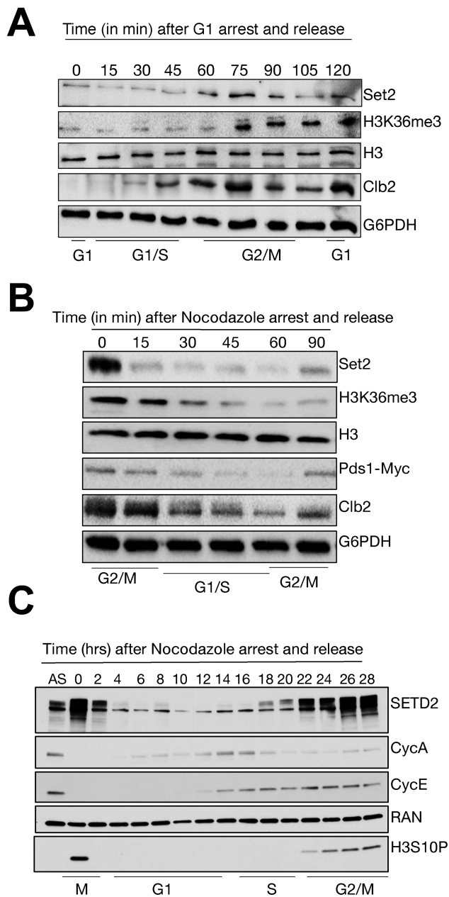
Figure 5. Yeast and human Set2 are cell cycle regulated proteins. (A) Set2 protein is cell cycle regulated. WT and set2Δ cells were arrested in the G1 phase using \alpha -factor and released into fresh medium. Whole cell extracts were prepared at indicated time points and probed for Set2, H3, H3K36me3, Clb2 (marker for cell cycle progression) and G6PDH (total protein loading). (B) Set2 protein levels are down-regulated during progression through mitosis and mitotic exit. Whole cell extracts were prepared at designated time points after release from nocodazole. WT cells were released into fresh medium and immunoblotted for Set2, Clb2 (a marker for cell cycle progression), Pds1 (a marker for metaphase to anaphase transition) and G6PDH (total protein loading control). Analogous to Set2, H3K36me3 levels similarly change across the cell cycle, as analyzed by immunoblotting for H3K36me2/me3, and anti-H3 (loading control). (C) Human SETD2 is a cell cycle regulated protein. U2OS cells were synchronized using nocodazole, collected at indicated time points, and immunoblotted for SETD2. CycA, CycE and H3S10P serve as markers for different cell cycle stages, whereas RAN was used as a loading control.
