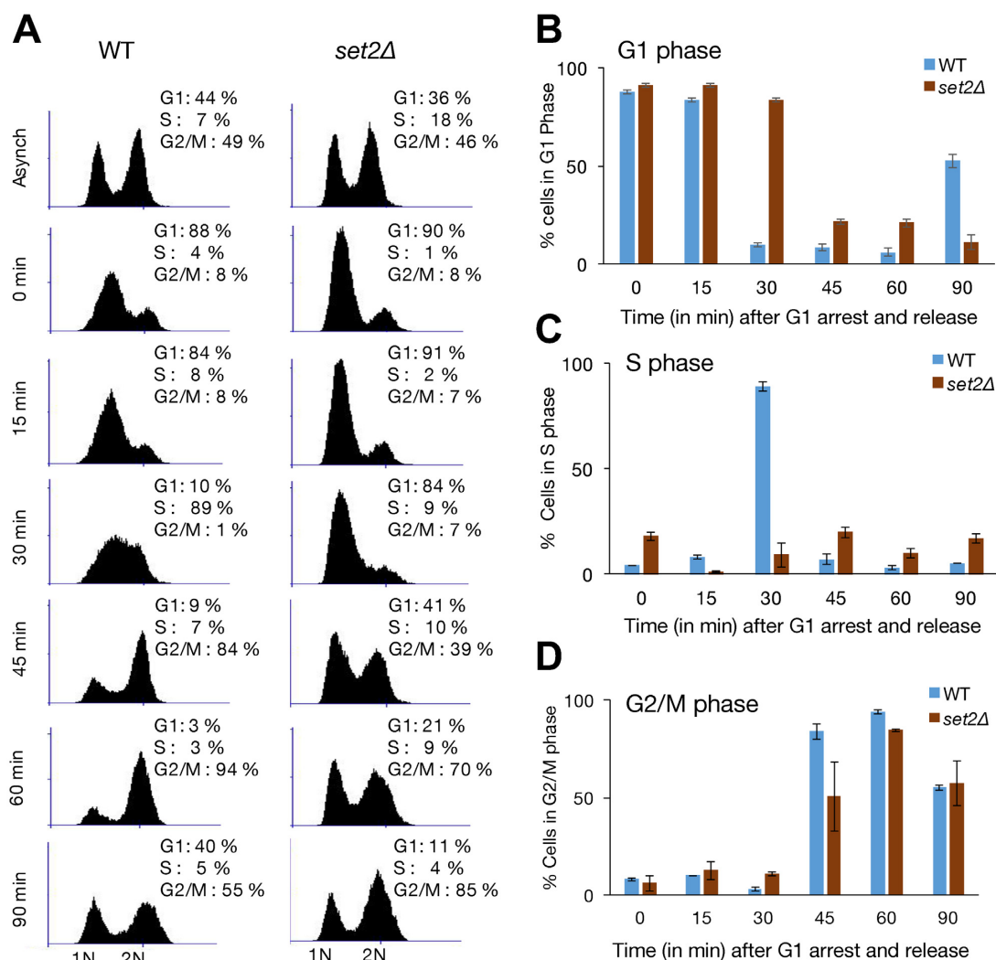
Figure 4. Loss of Set2 and H3K36 methylation abrogates yeast cell cycle progression. (A) Representative flow cytometry profiles of WT and set2Δ cells after \alpha -factor arrest and release, which reveal defects in the ability of set2Δ cells to properly progress through the cell cycle. Comparison of the profiles at 30, 45 and 60 min after release in G1 show set2Δ cells have a delayed entry into S-phase, which then progresses faster than that observed for WT cells. (B–D) Quantification of multiple flow cytometry profiles of WT and set2Δ cells ( n > 3 ) in which G1, S and G2/M cells from WT and set2Δ cells are counted.
